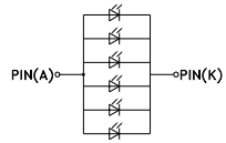
BLU CIRCUIT DIAGRAM IF=20mA VF=2.8-3.2V
