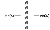
BLU CIRCUIT DIAGRAM IF=20mA VF=2.8-3.2V
